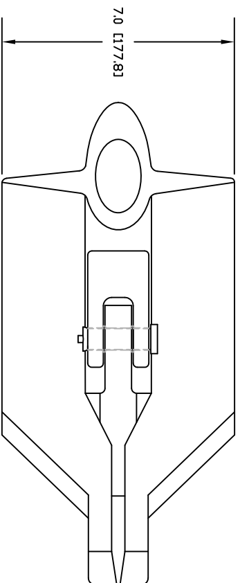
TOP VIEW
